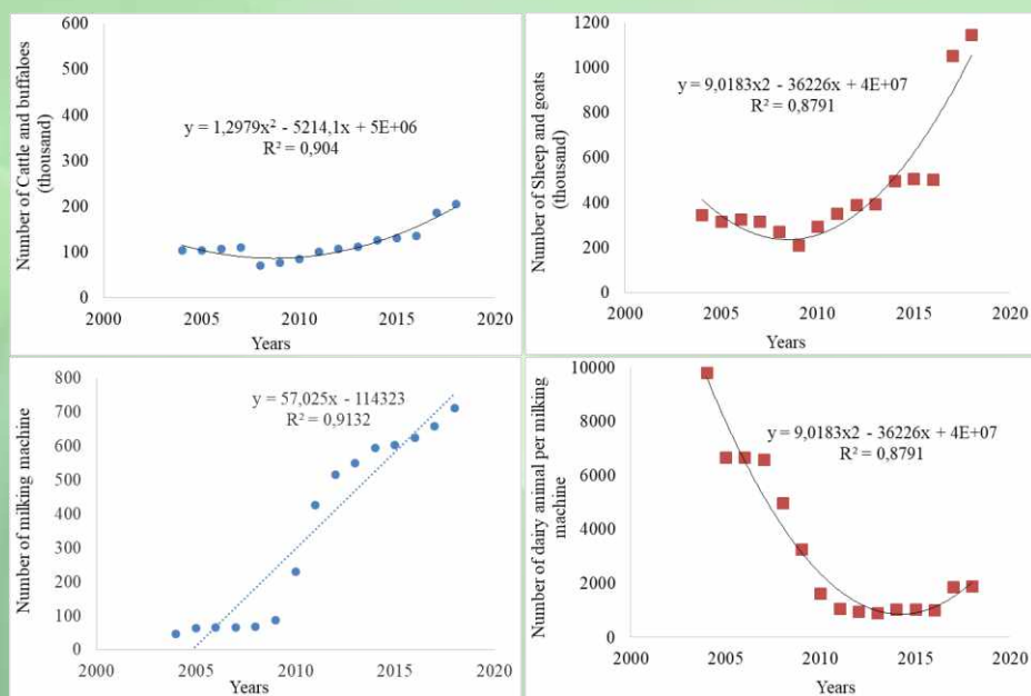
Figure 3. The change in the number of dairy animal and the number of dairy animals per milking machine in Diyarbakır province of Turkey since 2002 (TUİK, 2019)
